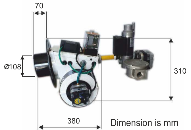
Burner Dimension
